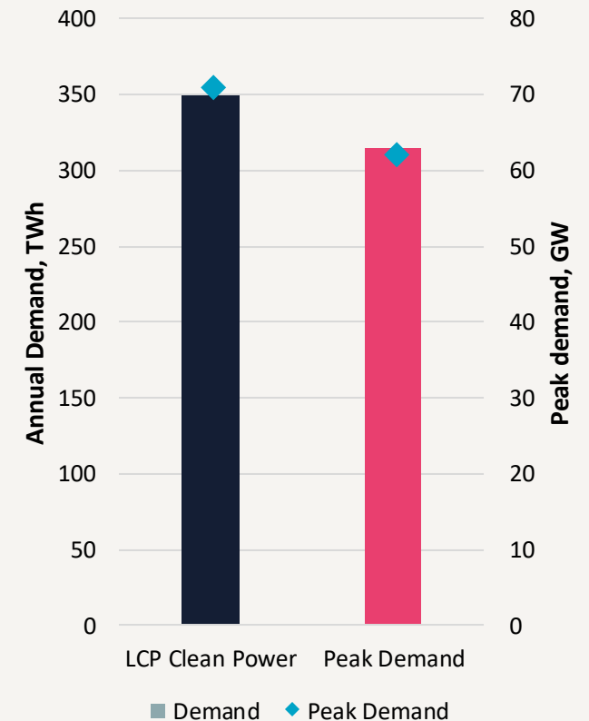
Demand comparison between LCP Delta Clean Power Scenario and NESO Clean Power Scenario
