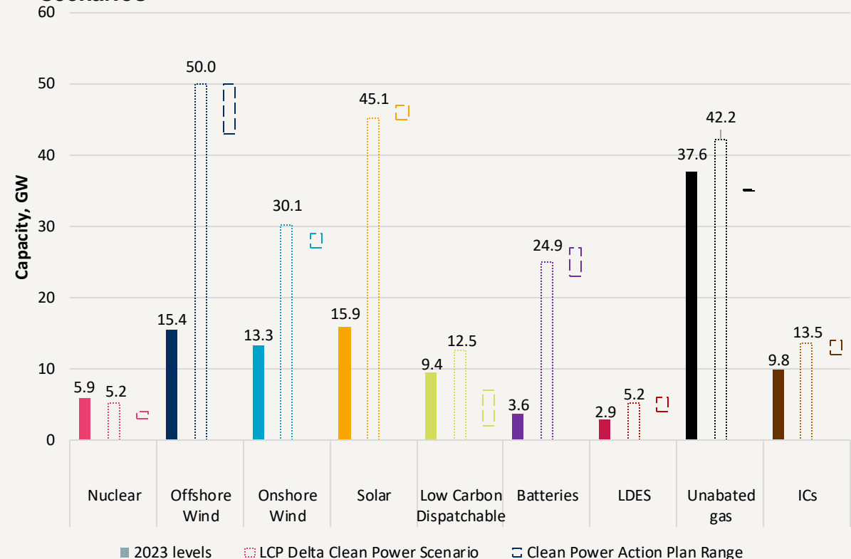
Installed capacity in 2030 under DESNZ and LCP Delta Clean Power scenarios
